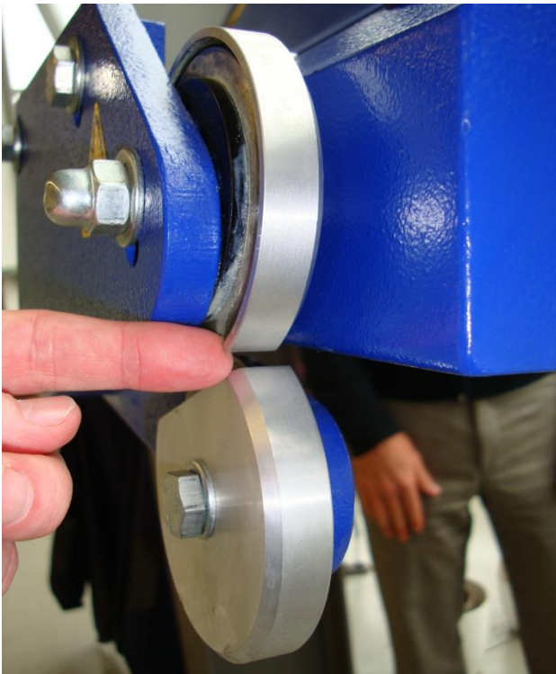
Figure 13: Example of finger-safe cutting device
