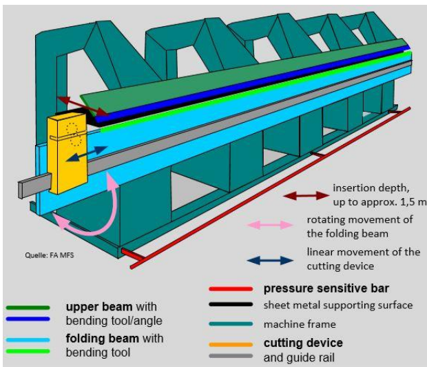
Figure 6: Long folding machine with power-operated cutting device (orange), limited insertion depth and an emergency stop pressure sensitive bar (red)
