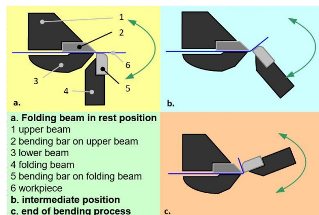
Figure 2: Principle folding, rotating movement
