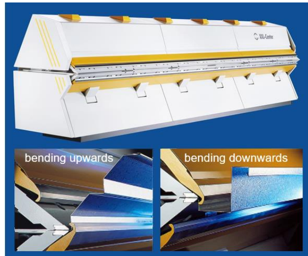
Figure 8: Example of a long folding machine with two folding beams, i. e. bending upwards and bending downwards
